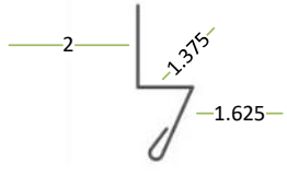
BD3 Base Drip Angle 2
