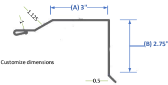
RGR4 Residential Gable Rake 3x2.75
