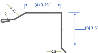
RGR5 Residential Gable Rake
