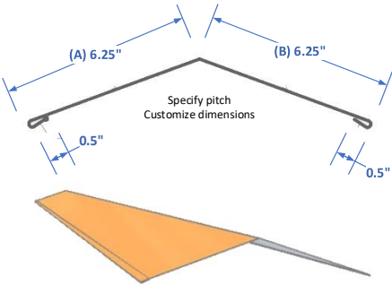
RCA Flat Ridge Cap
