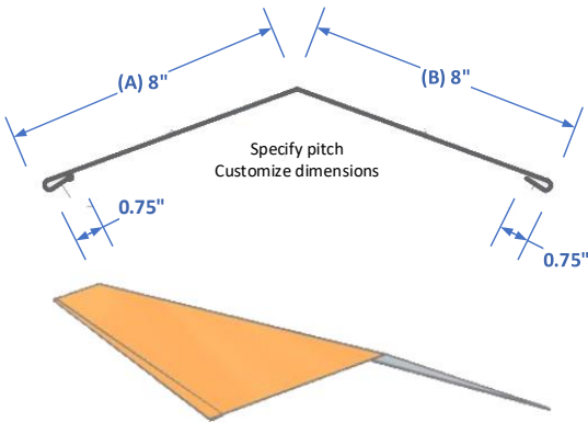
RCA18 Flat Ridge Cap
