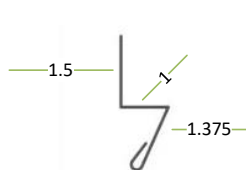
BD1 Base Drip Angle 1.50
