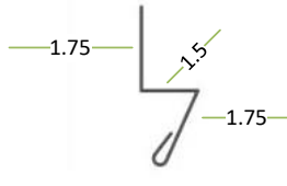
BD2 Base Drip Angle 1.75
