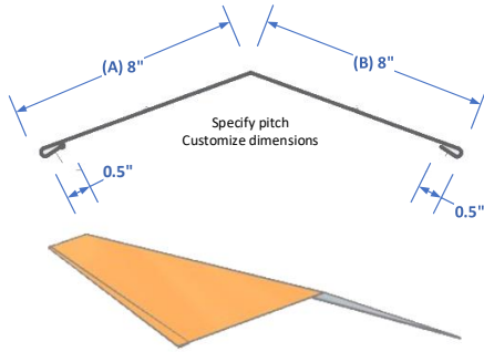
RCA16 Flat Ridge Cap
