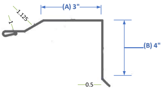
RGR3 Residential Gable Rake 3x4
