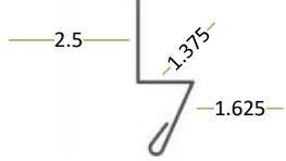
BD4 Base Drip Angle 2.5
