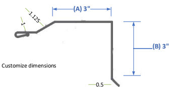
RGR1 Residential Gable Rake 3x3
