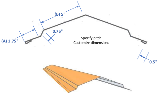
RCB Standard Ridge Cap
