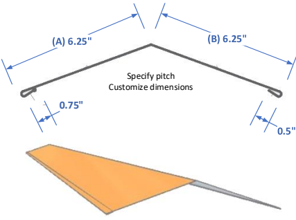
RCA14 Flat Ridge Cap
