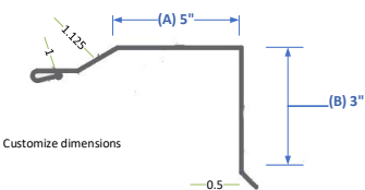
RGR2 Residential Gable Rake Large 5x3
